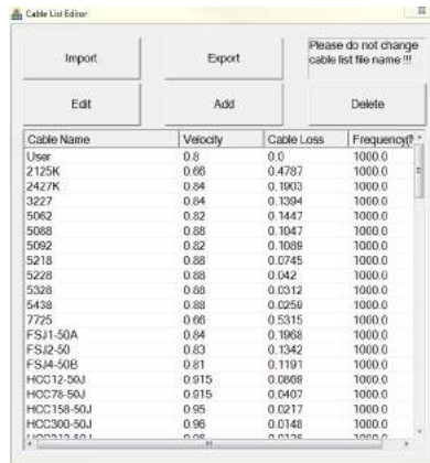
Figure 49 Cable List Editor
